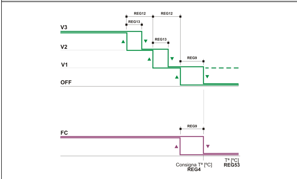
FC: Fan-coil
